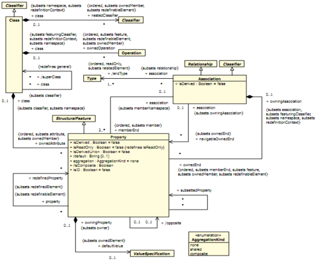
Figure 14.2 - Key concrete classes from UML2 Kernel package
