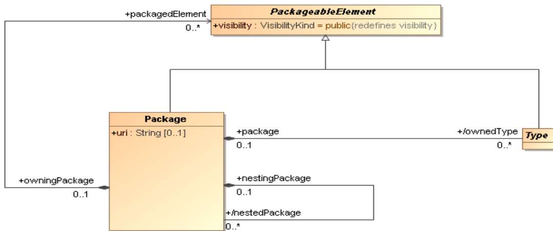
Figure 12.4 - EMOF Packages
