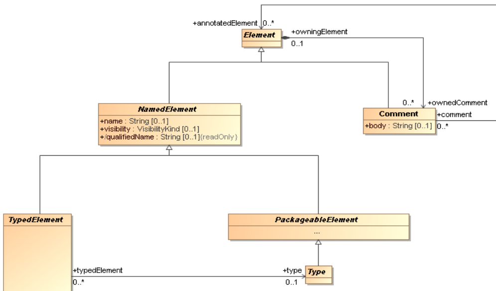
Figure 12.5 - EMOF Types
