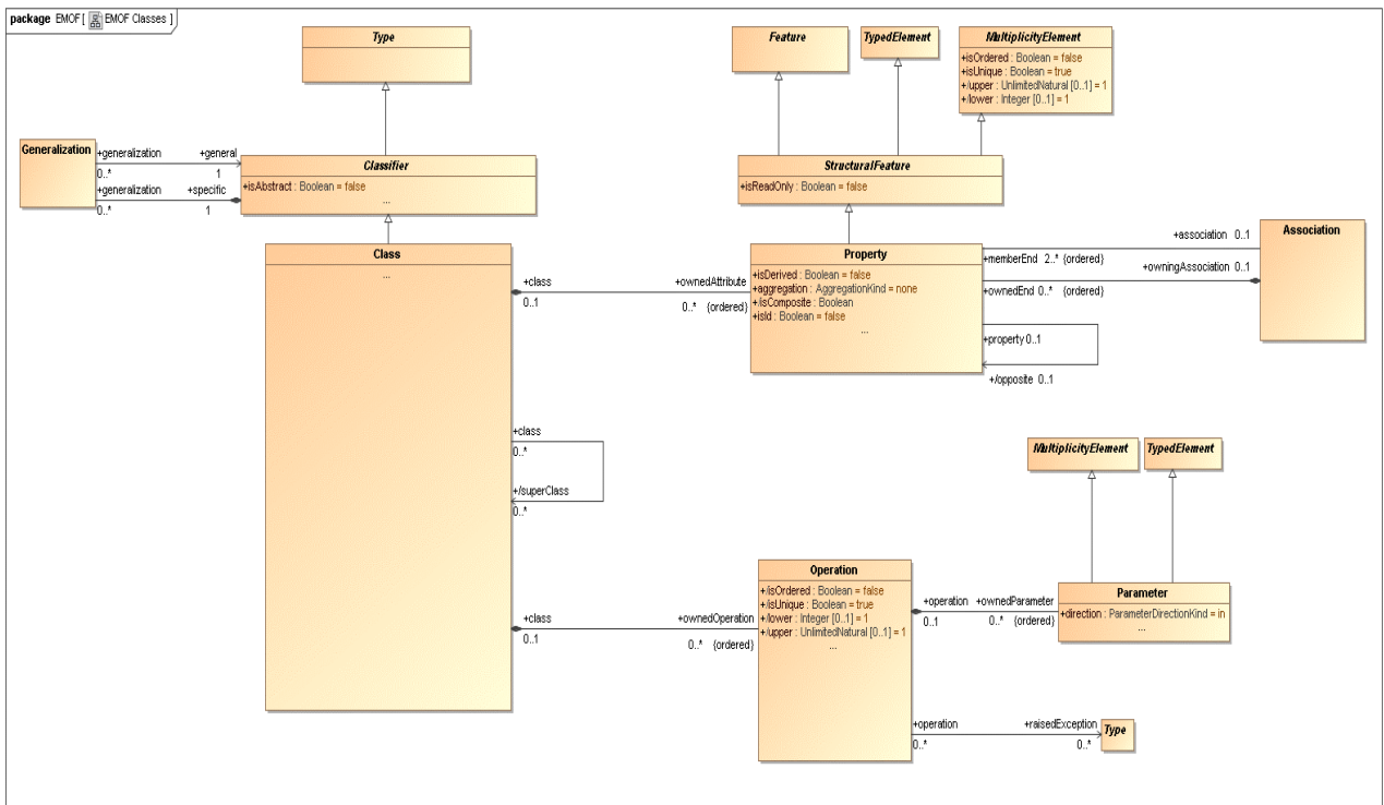
Figure 12.2 - EMOF Classes
