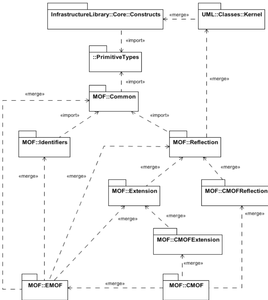
Figure 14.1 - CMOF Packages
